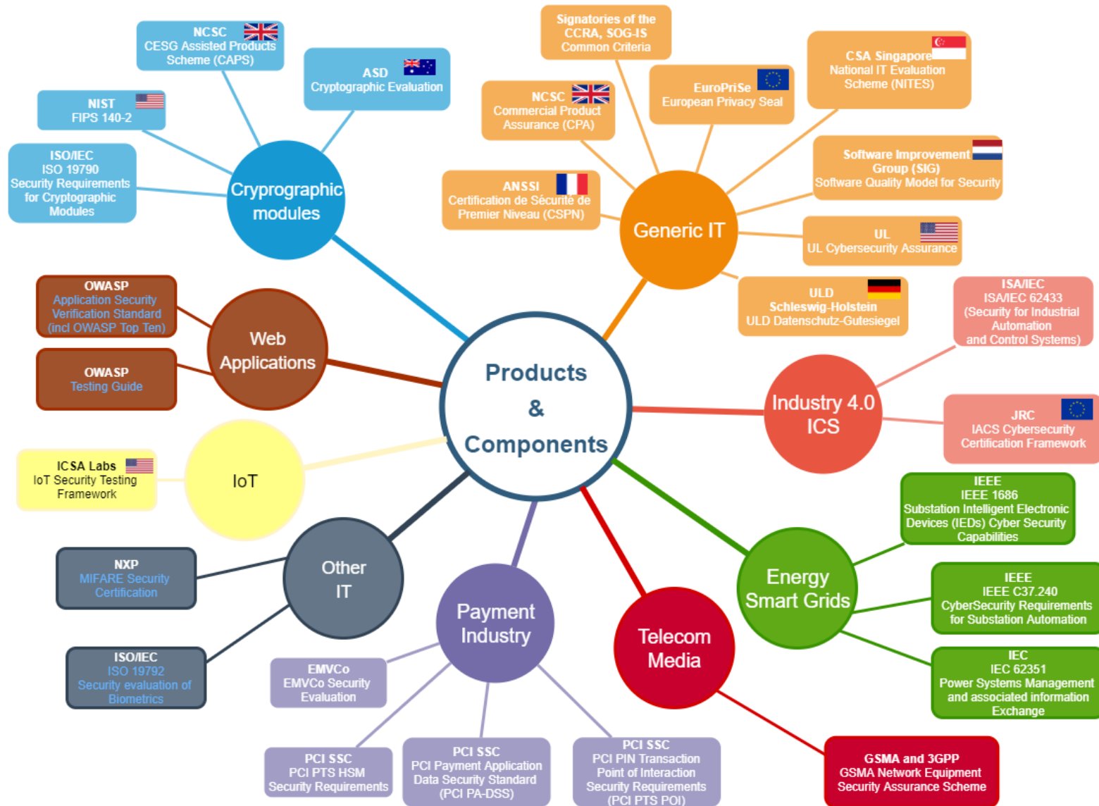
Figure 35: Standards and Frameworks - Products and Components
