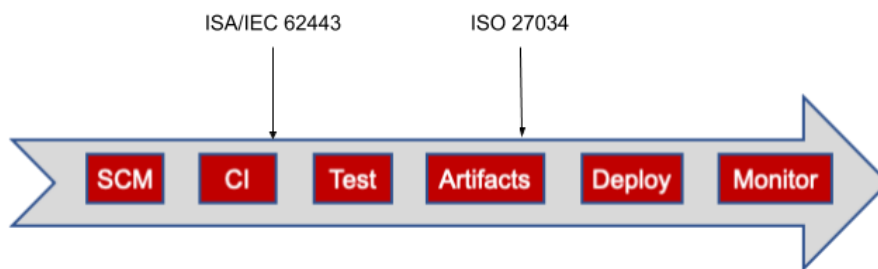
Figure 26: DevSecOps process certification
