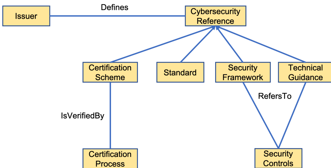
Figure 12: Main concepts for comparing cybersecurity certification schemes and standards
