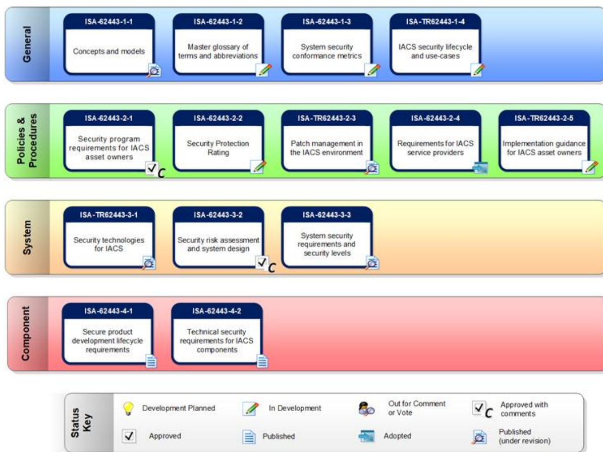
Figure 18: Status of the various work products in the ISA/IEC 62443 [59]
