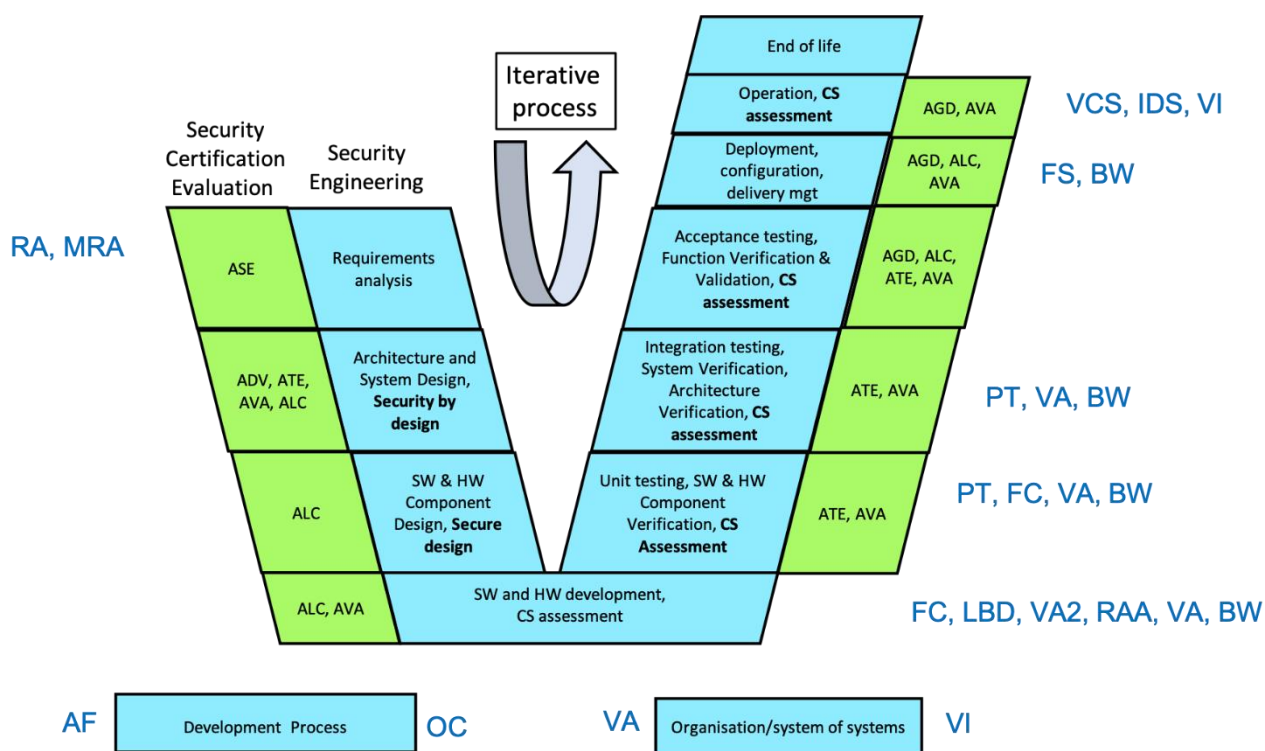
Figure 22: SPARTA Assessment tools and Certification Process
