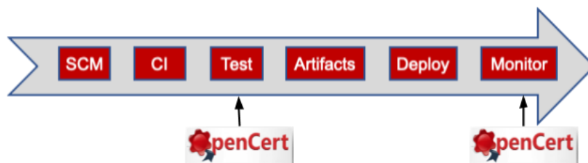
Figure 24: integration of OpenCert tool into continuous integration and deployment process
