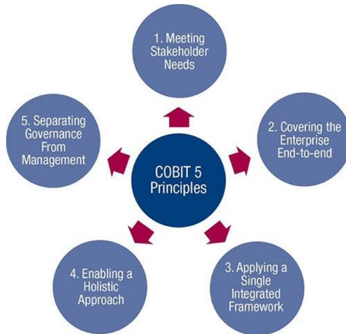
Figure 8: COBIT 5 Principles [35]
