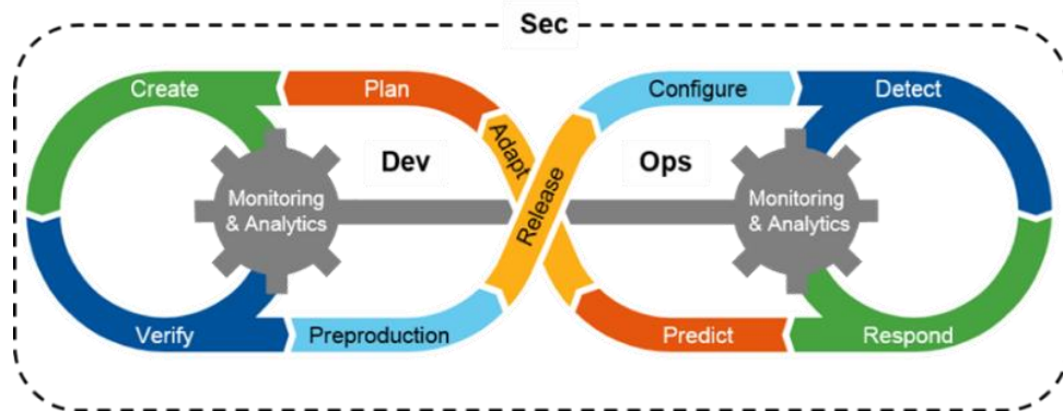
Figure 7: DevSecOps lifecycle [30]
