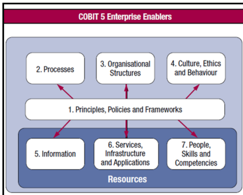
Figure 9: COBIT 5 Enablers [36]
